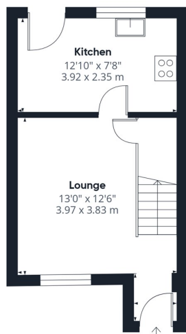
Ground Floor Building 1
